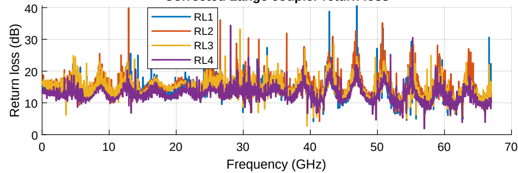
Corrected Lange coupler return loss
